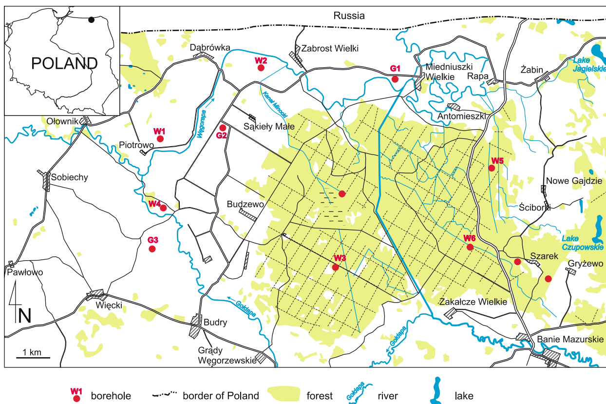
Fig. 1. Location of the studied profiles. W1, W2, W4 – analysed profiles
