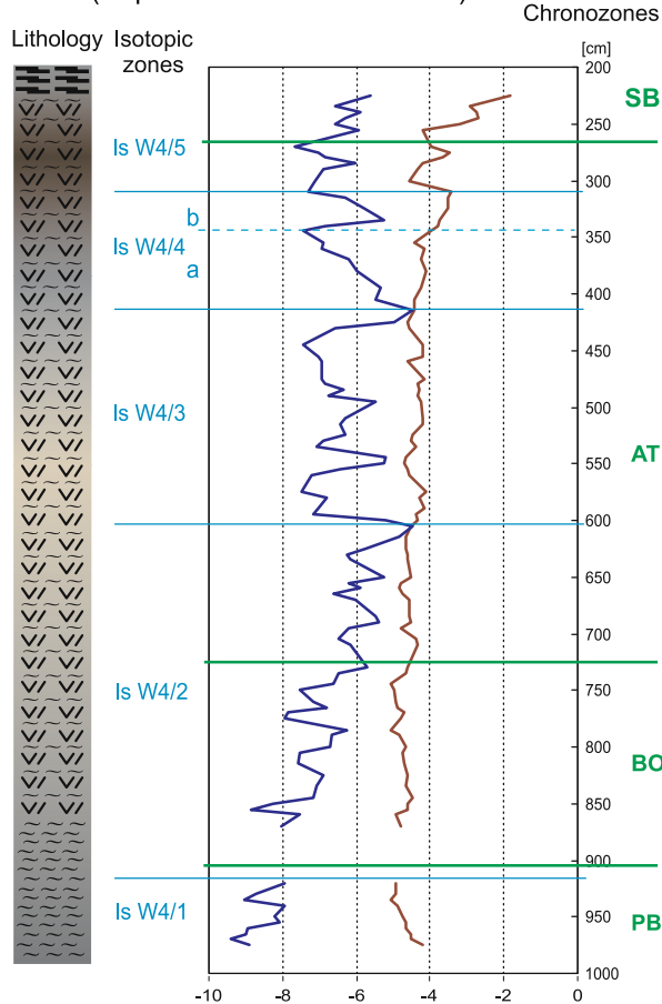
Fig. 2. Isotope curves of \delta^{18}\text{O} and \delta^{13}\text{C} and isotopic zones from: A – the W1 profile (Piotrowo-Lawniki); B – the W2 profile (Sakiety Małe); C – the W4 profile (Budzewo)
